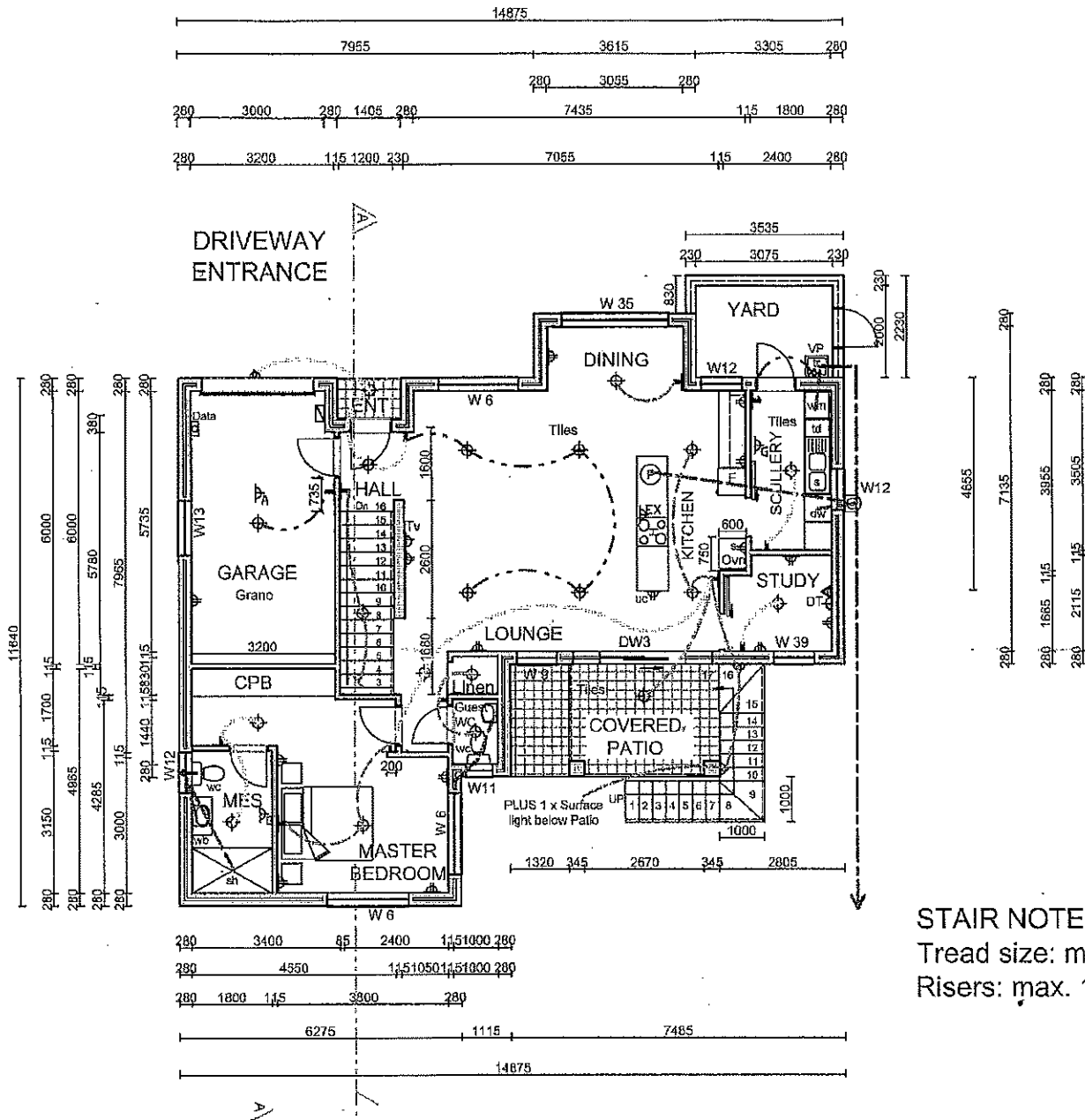
GROUND FLOOR PLAN 1:125 TYPE W2
