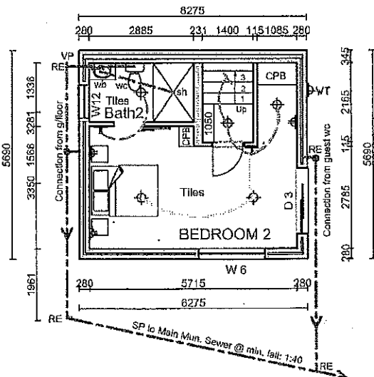
LOWER GROUND FLOOR PLAN 1:125 TYPE W2 (Kas, Ka7, Ka9, Ks1)
