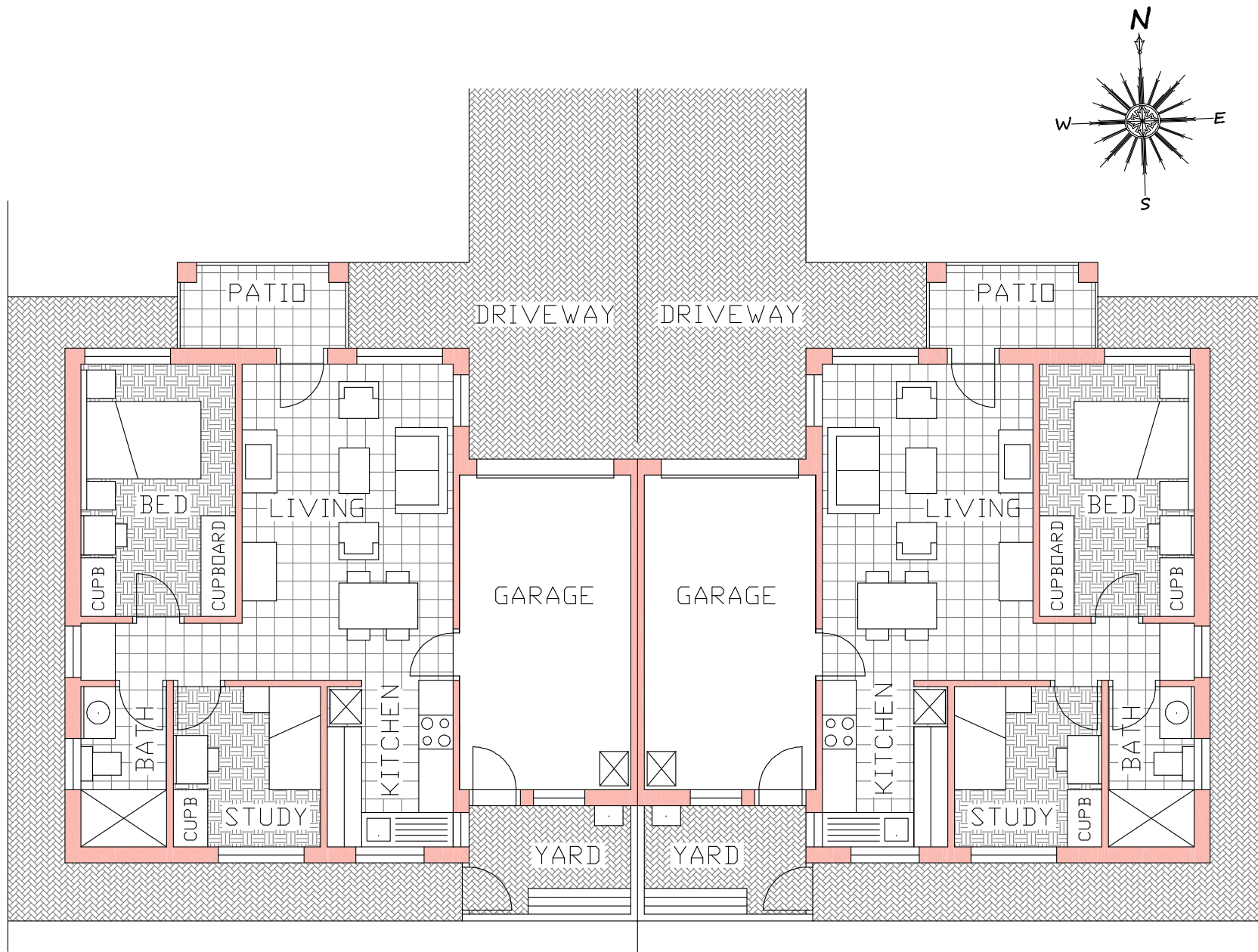
FLOORPLAN - TYPE E - 1:100 - 86m 2 GROENKLOOF RETIREMENT VILLAGE GEORGE
